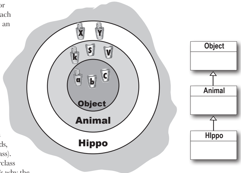
A single Hippo object on the heap
