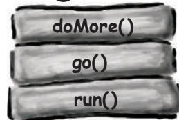
new thread
