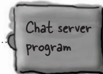
Server
