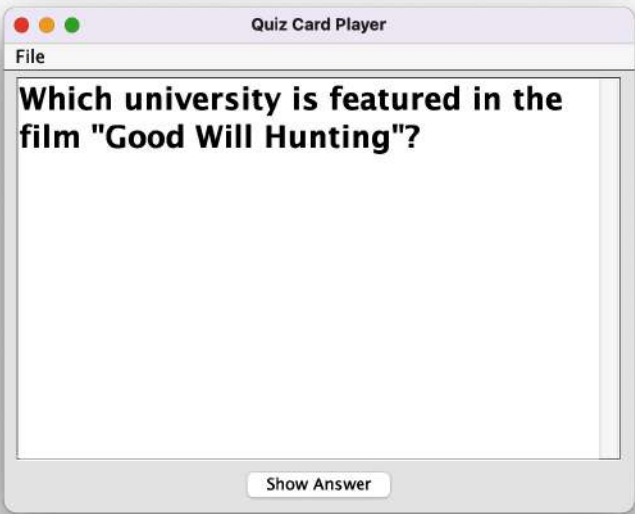
QuizCardPlayer
